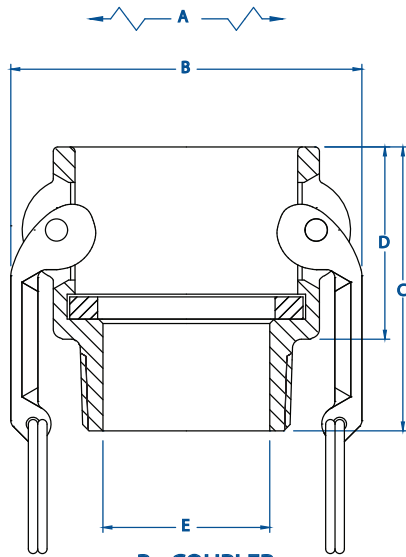
B - COUPLER
